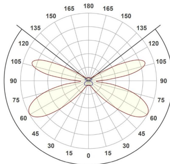
Measured light distribution curve, Ingemann Extruded LGP ■ C0/C180 ■ C90/C270
