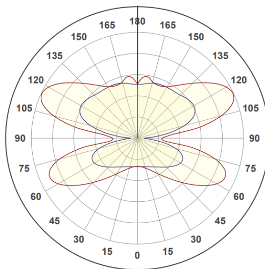
Measured light distribution curve, Cast Lumina LGP ■ C0/C180 ■ C90/C270
