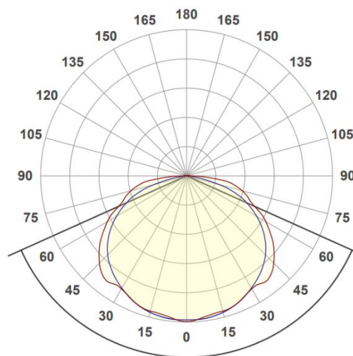
Measured light distribution curve, Ingemann Light Guide Bend
