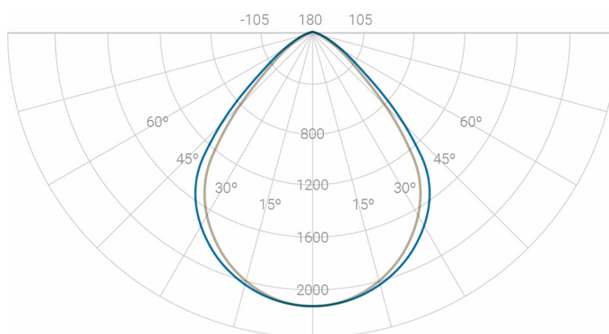
Measured light distribution curve, temilux®ID Pure ■ C0/C180 ■ C90/C270
