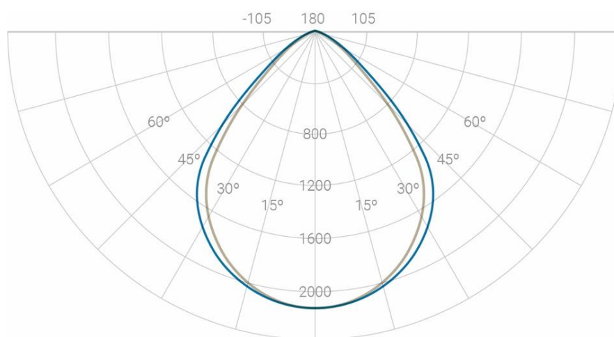
Measured light distribution curve, temiluxID Pure
