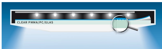
BASF D40 diffusor with microstructures facing away from LEDs for homogenic light.
