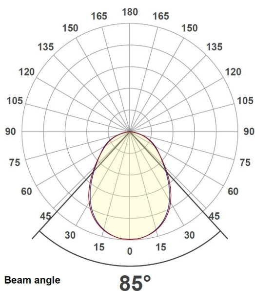
BASF D40 diffusor with microstructures facing away from LEDs for homogenic light.
