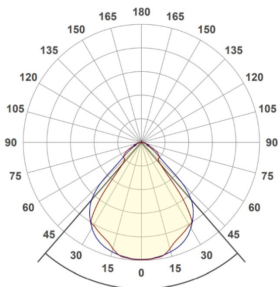
Measured light distribution curve, Ingemann Linear Prism ■ C0/C180 ■ C90/C270
