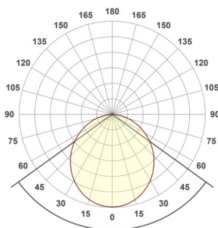
Measured light distribution curve, Ingemann Sky 60
