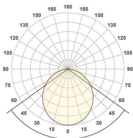
Measured light distribution curve, I-Fusion L1
