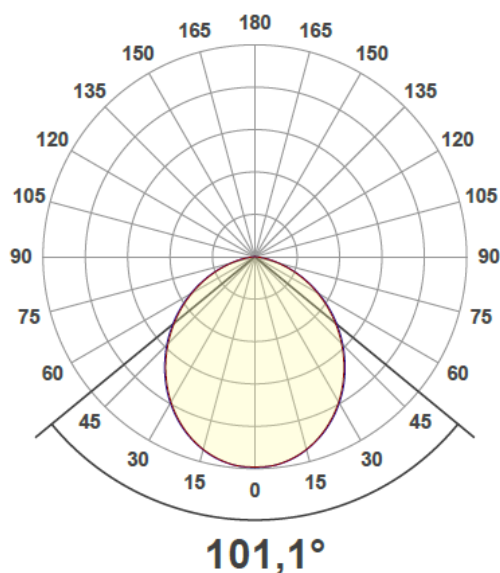
Measured light distribution curve, Lumieo S84
